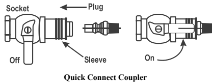
Quick Connect Coupler
